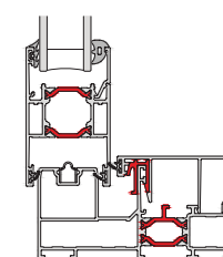
Mono Rail
