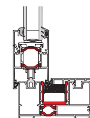
Duo Rail
