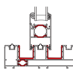
Tri Rail
